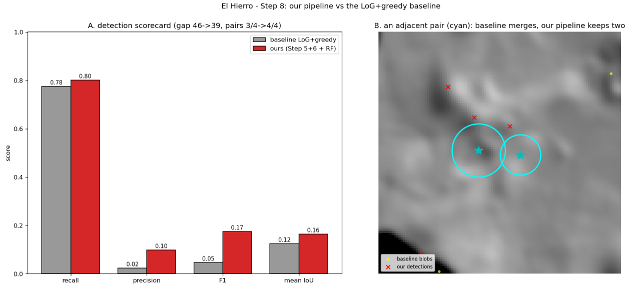
Figure 13: Step 8 on El Hierro. A : detection scorecard — the pipeline (red) beats the LoG + greedy baseline (grey) on recall, precision, F1 and IoU. B : a touching pair (cyan): the baseline blobs (yellow) collapse onto one cone, while our detections (red crosses) keep one on each.
