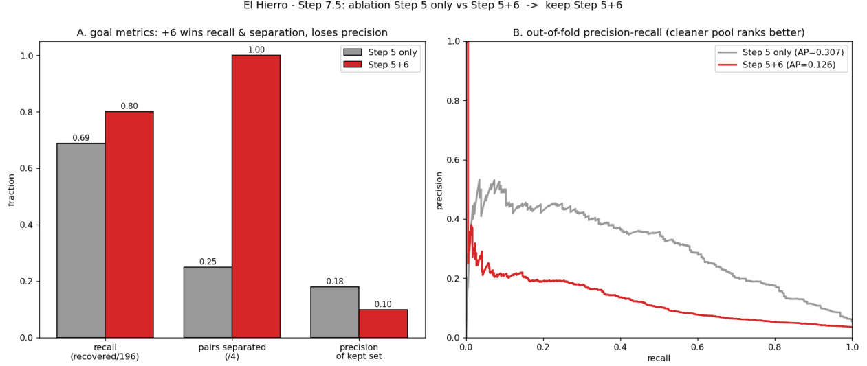
Figure 12: Step 7.5 on El Hierro. A : goal metrics — adding Step 6 (red) raises recall and takes pair separation from 1/4 to 4/4, while lowering the kept-set precision. B : the Step-5-only pool is cleaner and ranks better (higher AP), but cannot cover the merged cones; the union is the pool that delivers the separation.
