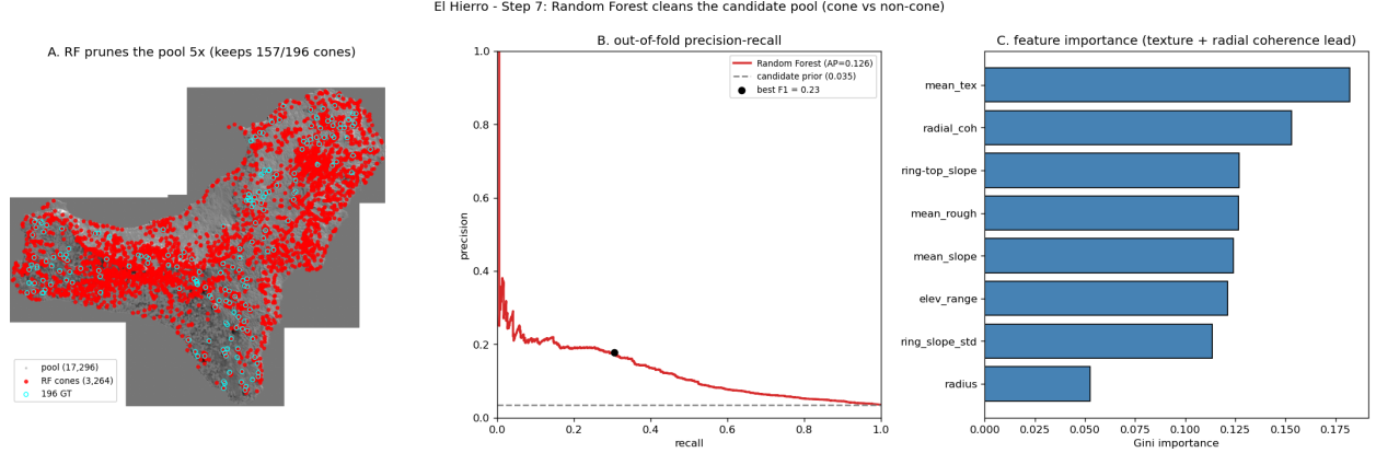
Figure 11: Step 7 on El Hierro. A : the Random Forest prunes the union pool \sim 5\times (grey: all 17,296 candidates; red: the ones kept; cyan: the 196 ground-truth craters). B : out-of-fold precision–recall curve ( AP = 0.126 ) well above the candidate prior (0.035). C : feature importances — texture and radial aspect-coherence lead.
